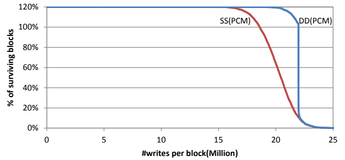
Fig. 3. Lifetime of PCM blocks with BCH-20 and 10% failure frequency threshold. “DD” denotes data dependent sparing and “SS” static sparing.
