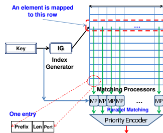
Fig. 1. The basic CA-RAM Architecture
